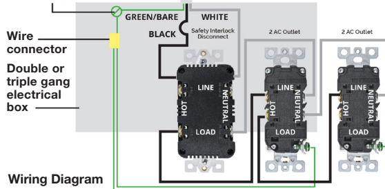
Grounding connection box (if box has a grounding terminal)
